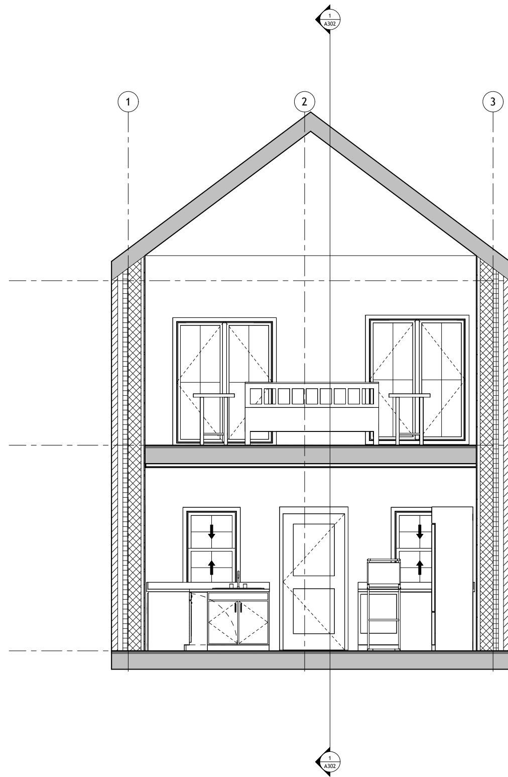
1 Section 1 1/2" = 1'-0"
